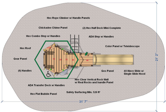
Fairview • PS-HVP-FAIRVIWa • Safety Zone: 30' x 21' • Installation Required
